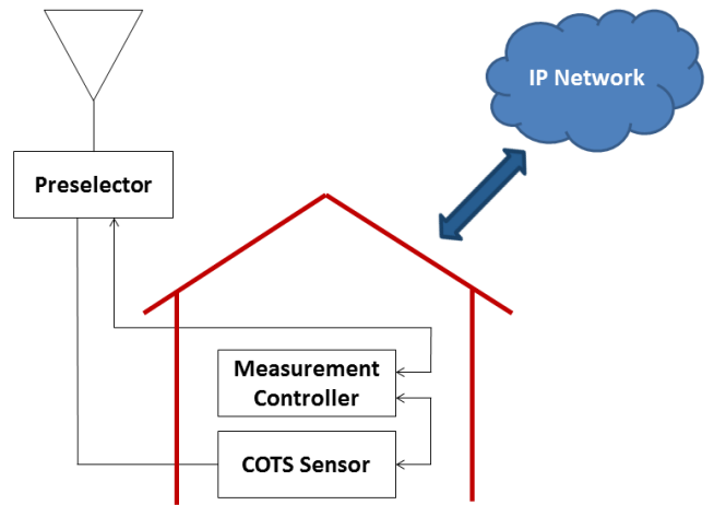
Fig. 9. General sensor architecture
